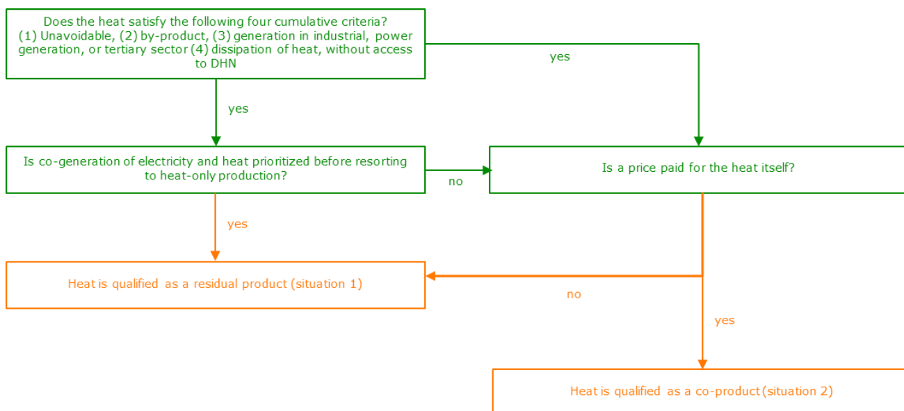
Figure 6 Decision tree heat from third parties
